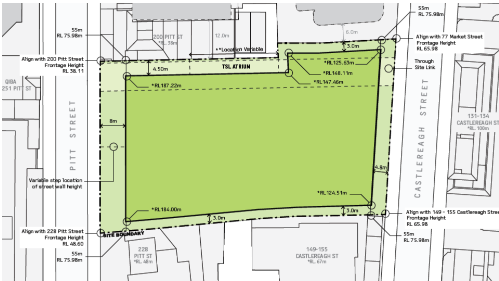
Figure 32 Building Setbacks – 55m – Maximum Height of Building (167.47m) Source: 3XN
